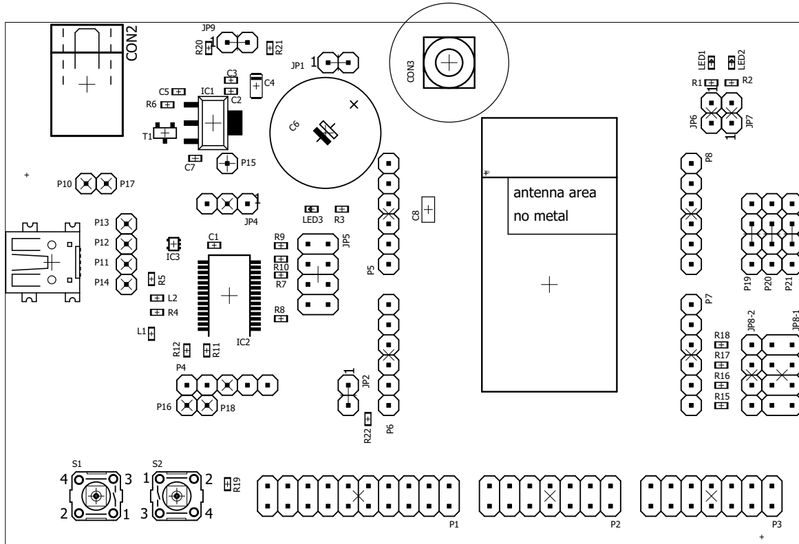
Figure 14: Assembly diagram
